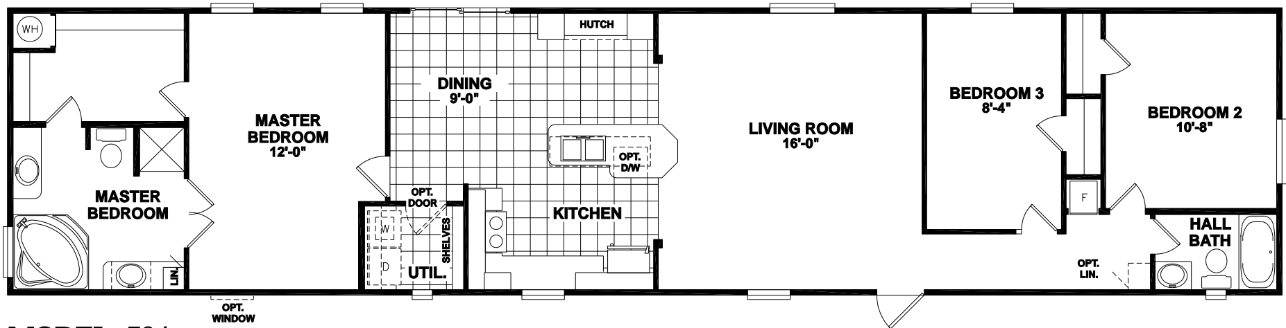
MODEL: 794 APPROX. 1304.67 SQ. FT. 3 BEDROOMS, 2 BATHS
